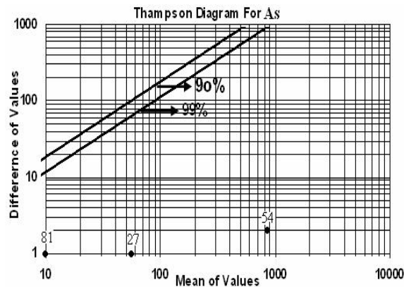
Figure 5: Shows Thompson diagram of as element
