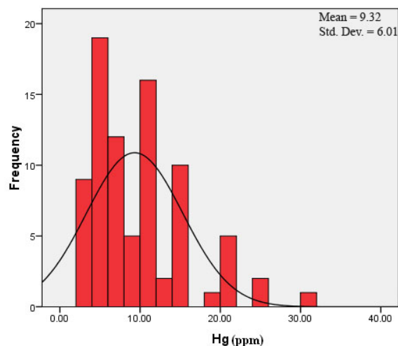
Figure 13- Frequency histogram of Hg element
