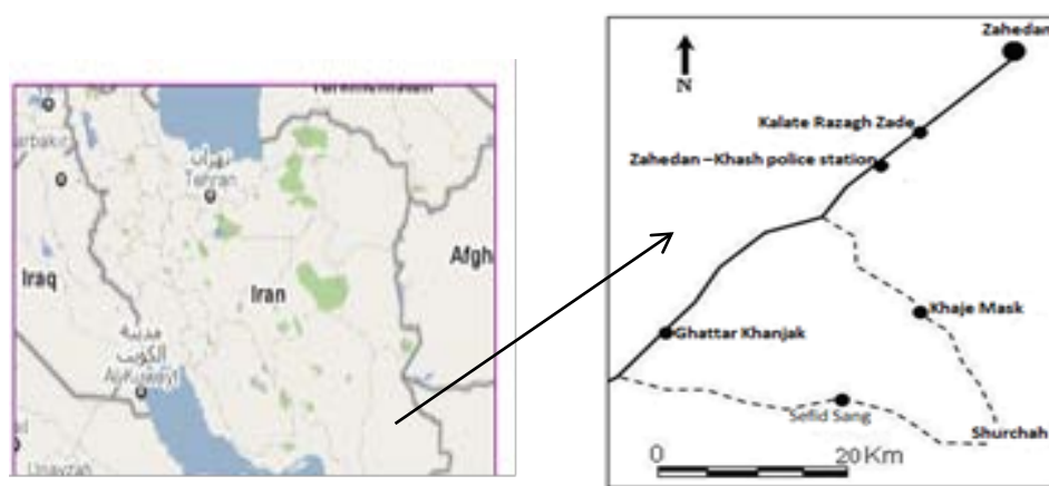
Figure 1: Geological location and the access roads to study area
