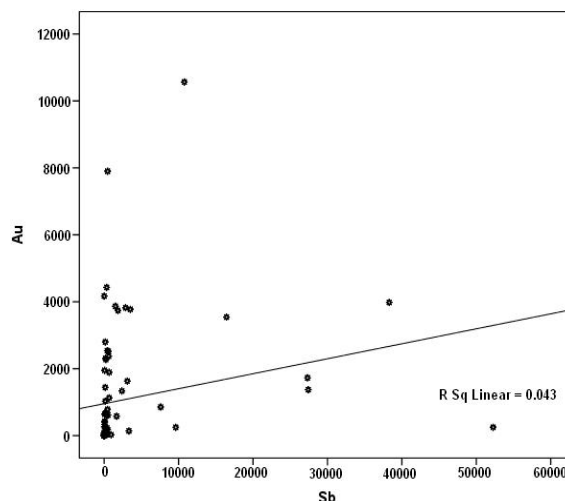
Figure 15: Shows dispersion of Gold with Antimony elements along with regression curve
