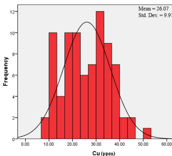
Figure 10- Frequency histogram of Cu element
