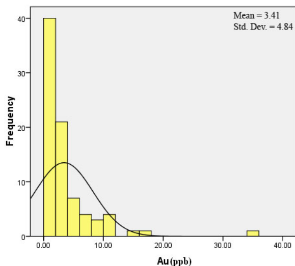
Figure 9- Frequency histogram of Au element
