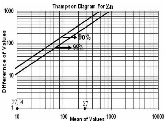
Figure 4: Shows Thompson diagram of Zn element
