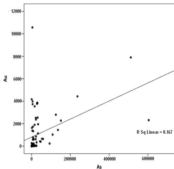
Figure 14: Shows dispersion of Gold with Arsenic elements along with regression curve
