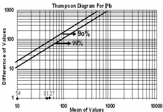
Figure 3: Shows Thompson diagram of Pb element
