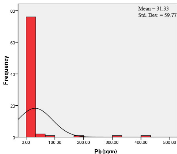
Figure 11- Frequency histogram of Pb element
