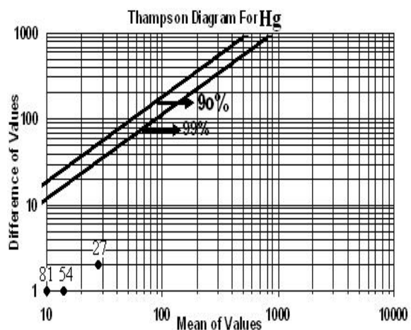
Figure 8: Shows Thompson diagram of Hg element
