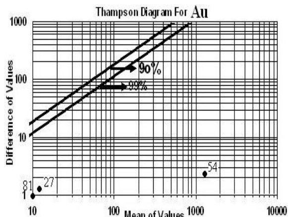
Figure 7: Shows Thompson diagram of Au element
