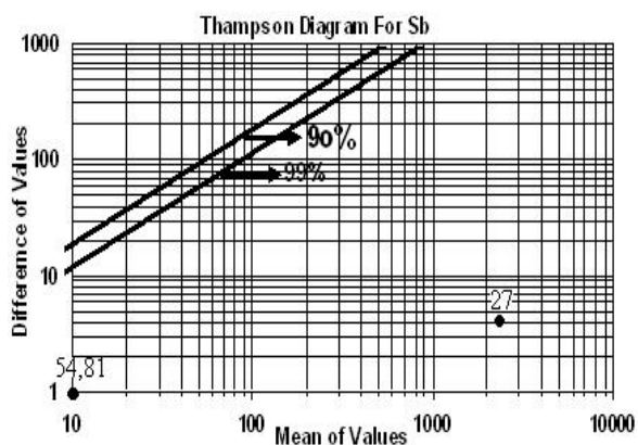
Figure 6: Shows Thompson diagram of Sb element
