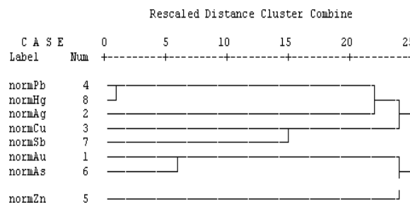
Figure 16- Shows Dendrogram related to stream sediments
