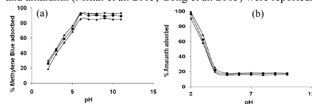
Figure 1a & b: Effect of pH on the methylene blue and amaranth adsorption respectively by tamarind pod shells (♦ 10 mg/L ■ 20 mg/L ▲ 50 mg/L)
