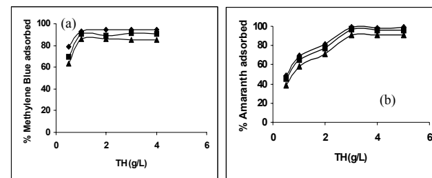
Figure 2a & b: Effect of adsorbent dosage on the methylene blue and amaranth adsorption respectively by tamarind pod shells (♦ 10 mg/L ■ 20 mg/L ▲ 50 mg/L)
