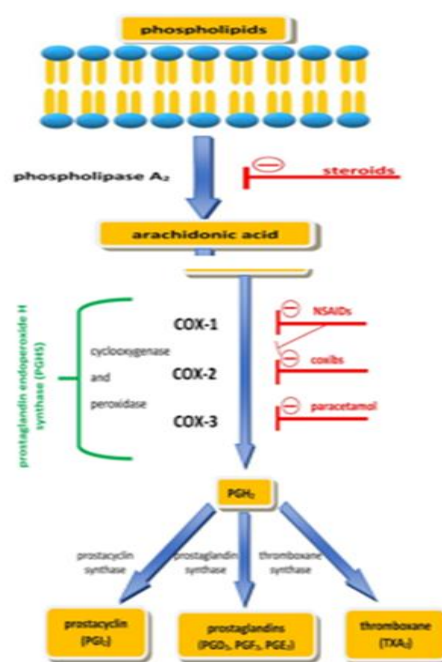
Figure 4. Cyclooxygenase mechanism
