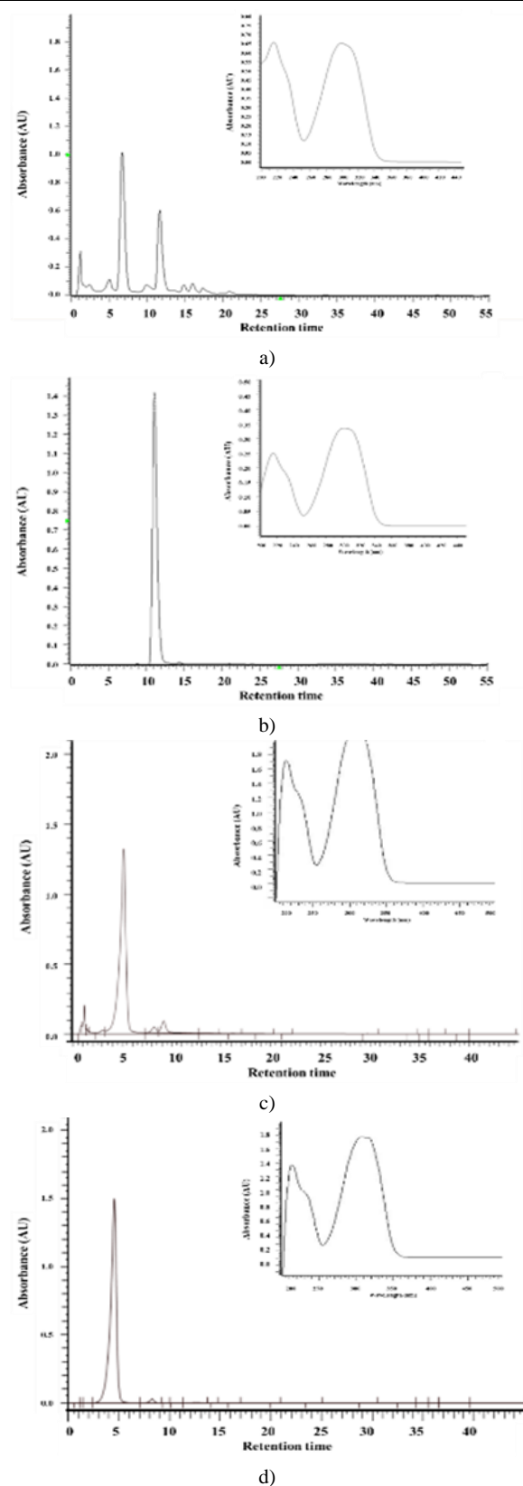
Figure 1. HPLC chromatograms and UV spectra of the ethylacetate subfraction F1 (a) and F1a (c) isolated from Polygonum cuspidatum root (a) and pure standard of resveratrol (b) and piceid (d)
