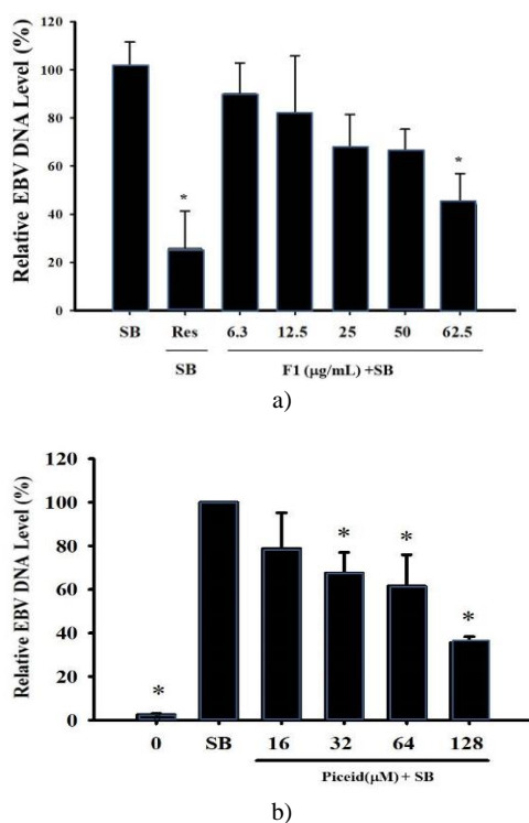
Figure 6. Inhibition Effects of F1 and piceid on EBV DNA replication
