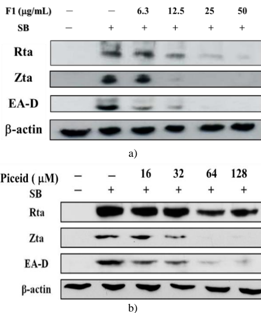
Figure 3. Inhibitory effects of F1 and piceid on the expression of EBV lytic proteins, including Rta, Zta and EA-D
