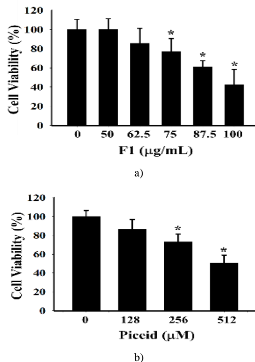
Figure 2. Toxicity of F1 and piceid on P3HR1 cells
