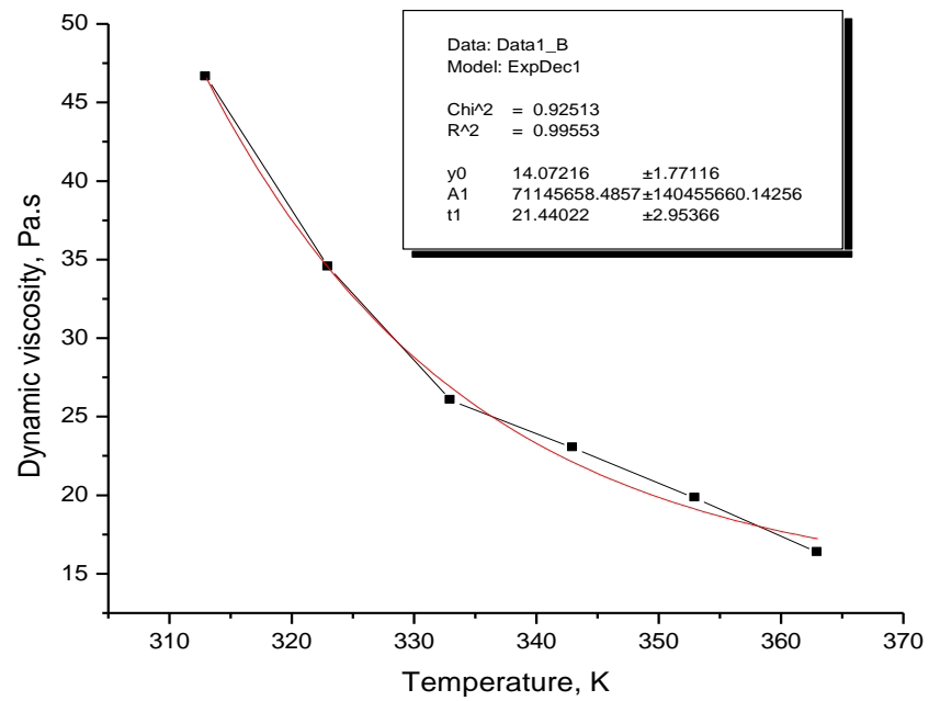
Figure 1. Dependence \eta = f(T) at shear rate 3.3\text{ s}^{-1}
