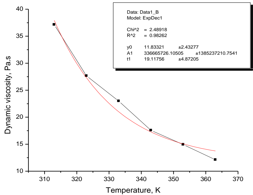
Figure 3. Dependence \eta = f(T) at shear rate 10.6s^{-1}
