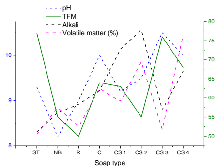
Figure 2. Comparison of synthesized soap properties with various commercial soaps
