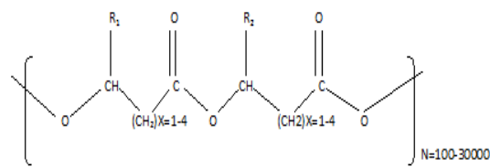
Figure 1. Polyhydroxybutyrate structure
