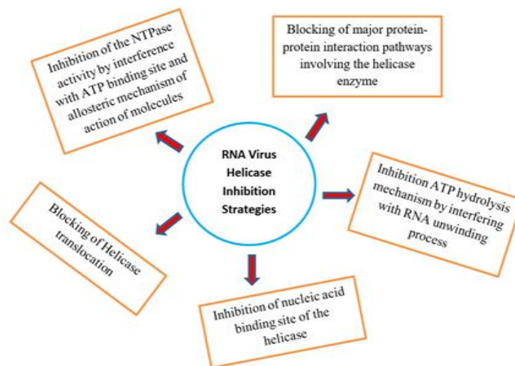
Figure 3. Strategies for inhibition of the viral RNA helicase enzyme by using potential drug molecules
