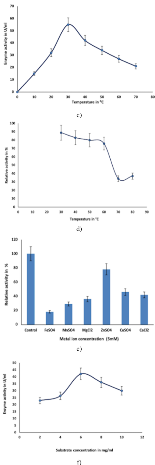
Figure 4. a, b, c, d) show the effect and stability of chitinase enzyme at different pH and temperature values respectively. E, f) show the effect of different metal ions (5mM) and substrate concentration respectively
