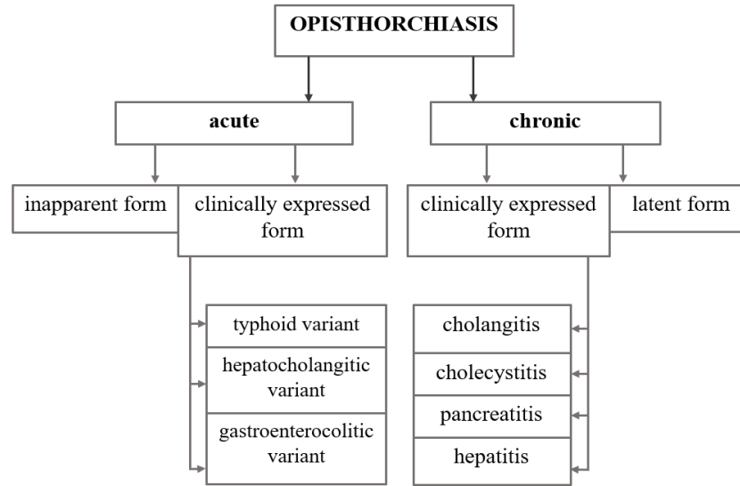
Figure 1. Clinical classification of opisthorchiasis (Belov & Feiginova, 1969)
