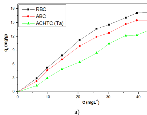
Figure 3. Variation of the adsorbed amounts of a) Cd, b) Mg ions versus phosphoric acid concentration
