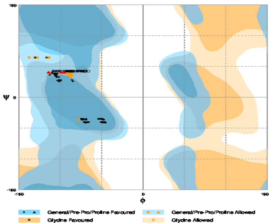
Figure 2. Ramachandran Plot for a given protein sequence(AIH14838)
