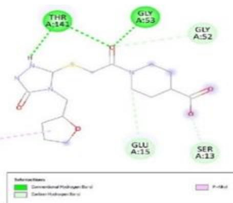
Figure 3. Ligand Binding site and interaction details
