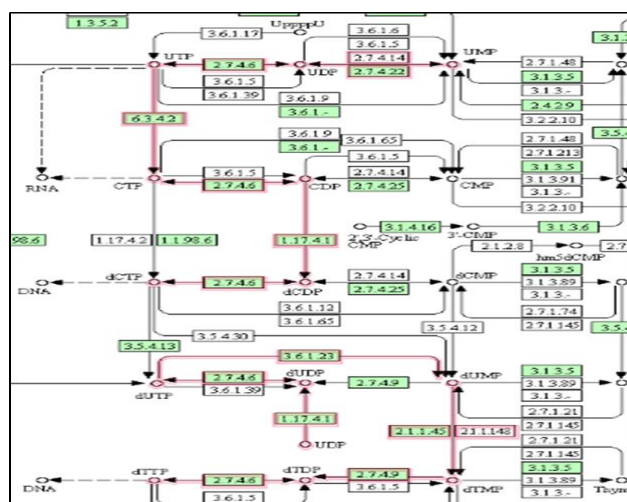
Figure 1. Screenshot of the active enzymes (highlighted in red) involved in the pyrimidine metabolism of Burkholderia pseudomallei
