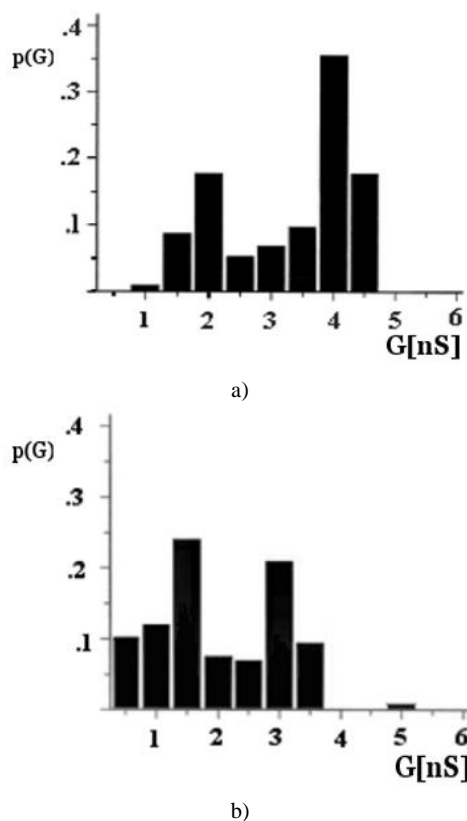
Figure 3. Histogram of conductance fluctuations of porin and EF-porin. The applied potential was +10 mV; T = 20^\circ\text{C} . Representation of the single channel conductance recordings peaks obtained with the EF-porin had two maxima at 1.5 and 3 nS (b) instead of 2 and 4 nS for the porin (a). p(G) , is the probability that the single channel conductance ( G ) is observed.
