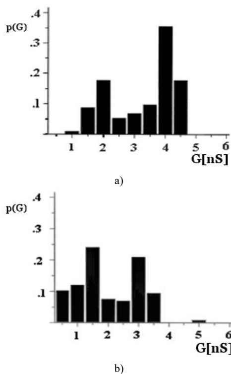
Figure 3. Histogram of conductance fluctuations of porin and EF-porin. The applied potential was +10 mV; T = 20^\circ\text{C} . Representation of the single channel conductance recordings peaks obtained with the EF-porin had two maxima at 1.5 and 3 nS (b) instead of 2 and 4 nS for the porin (a). p(G) , is the probability that the single channel conductance ( G ) is observed.
